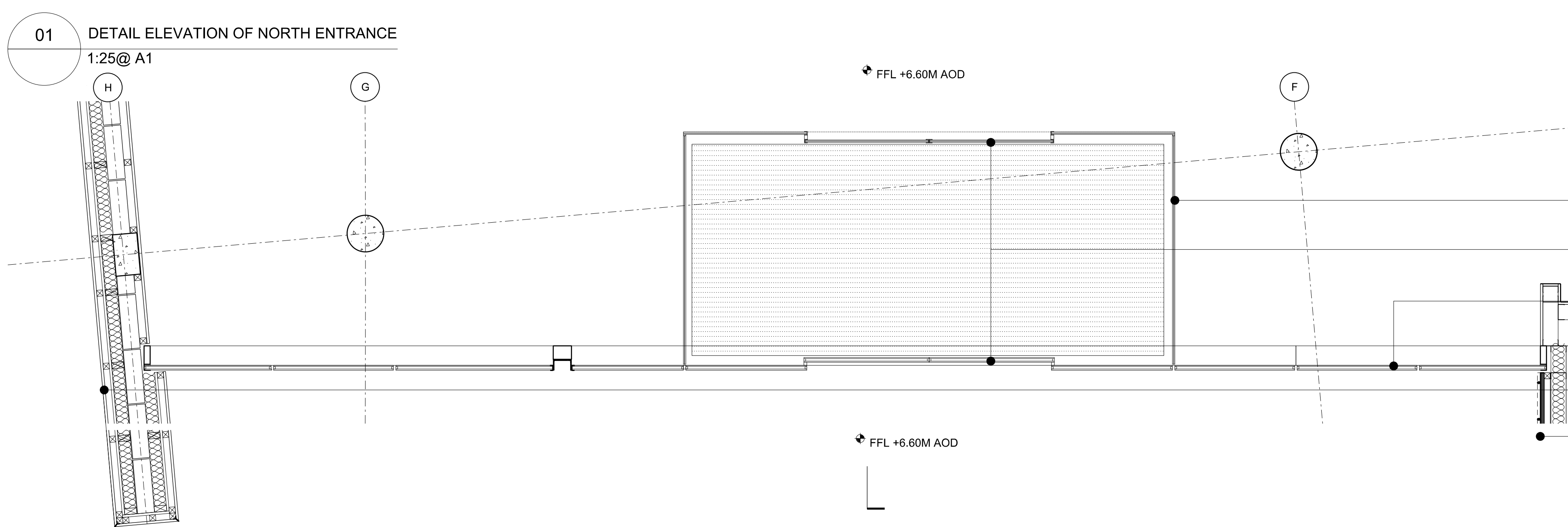
01 DETAIL ELEVATION OF NORTH ENTRANCE 1:25 @ A1 02 DETAIL PLAN OF NORTH ENTRANCE 1:25 @ A1
