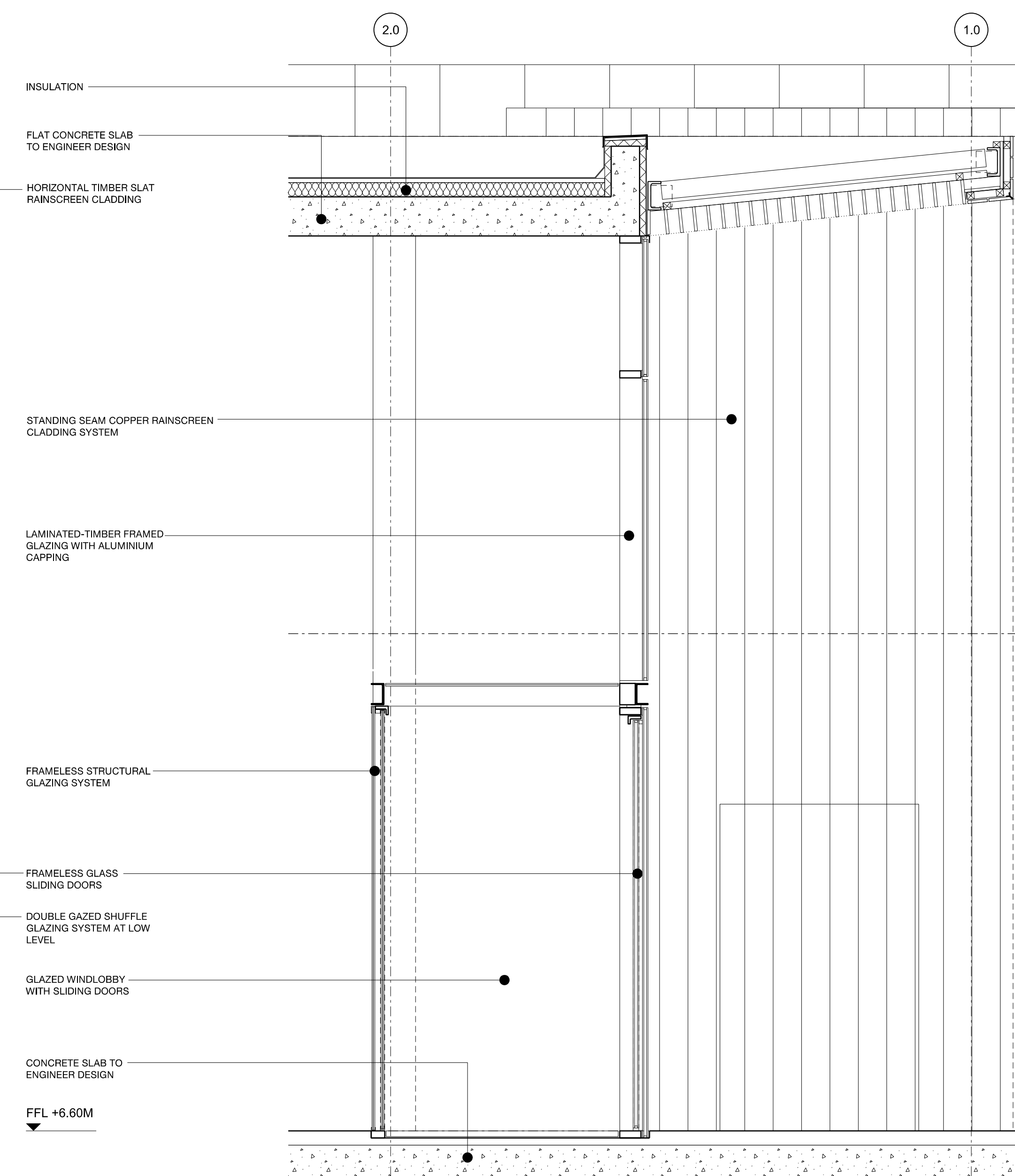
03 DETAIL SECTION THROUGH NORTH ELEVATION 1:25 @ A1
