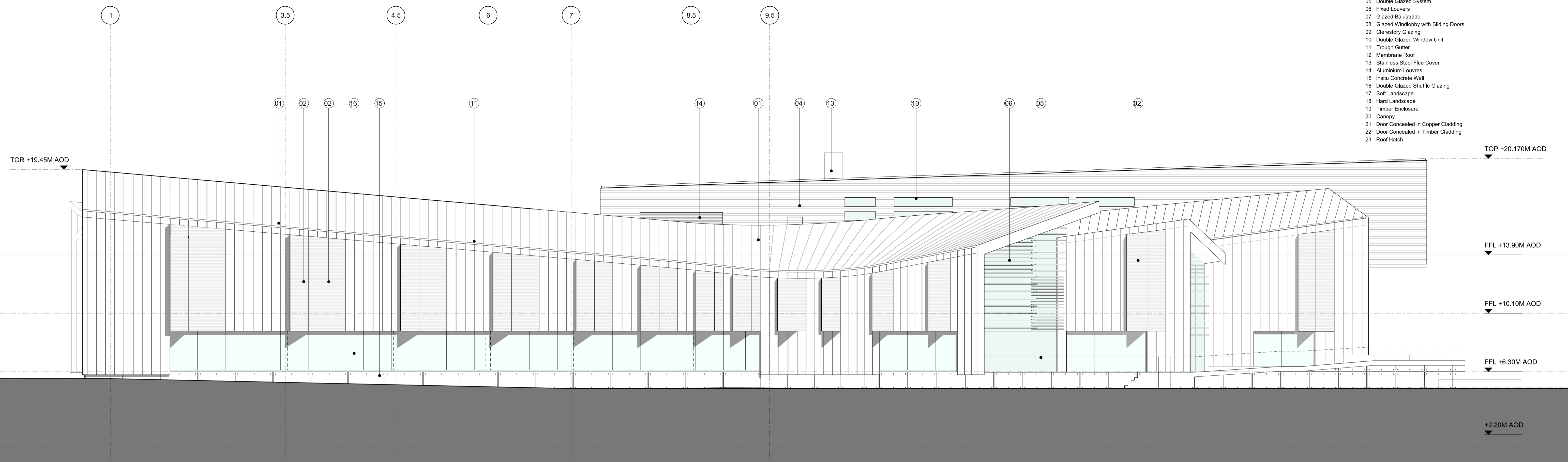
01 WEST ELEVATION
