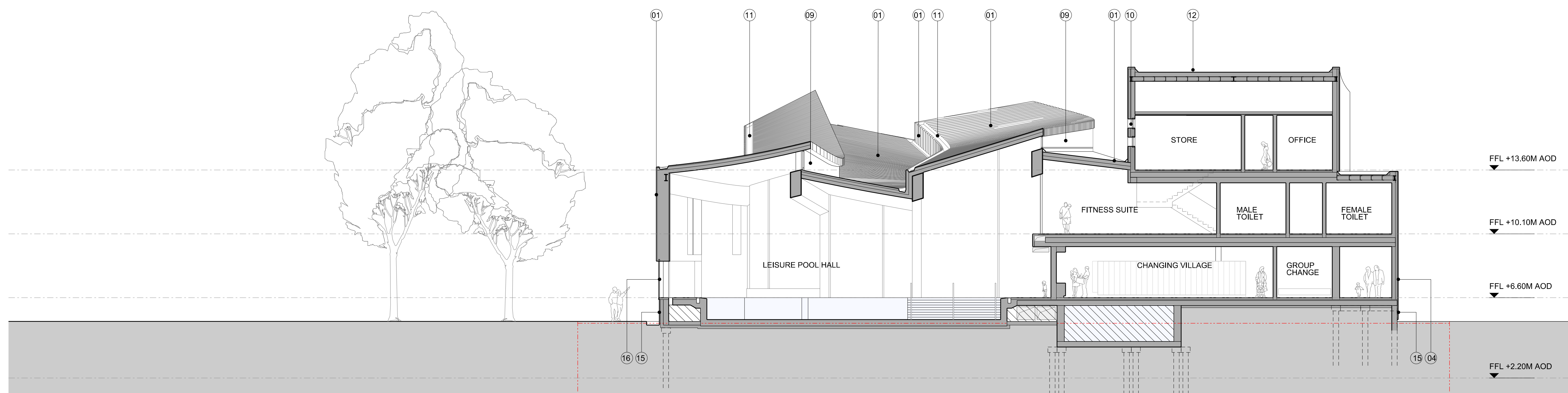
02 CROSS SECTION A-A
