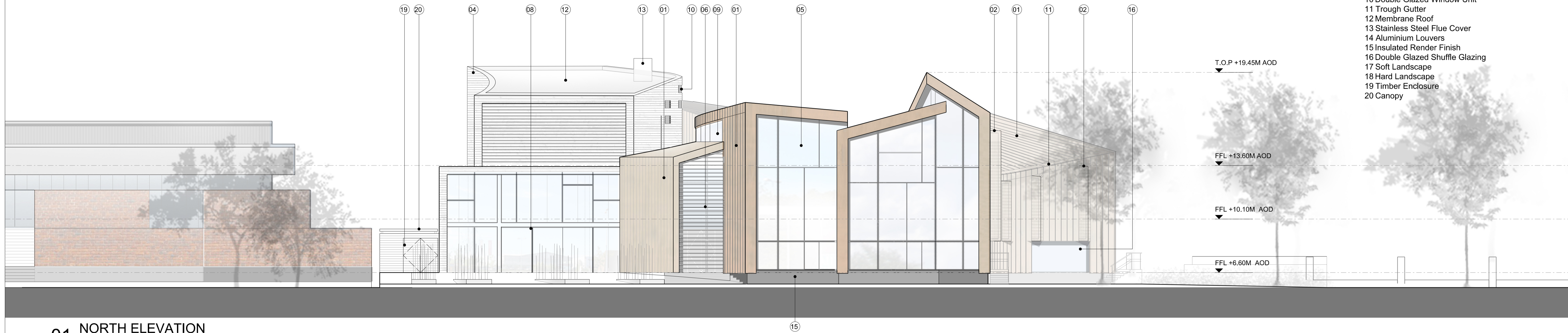
01 NORTH ELEVATION
